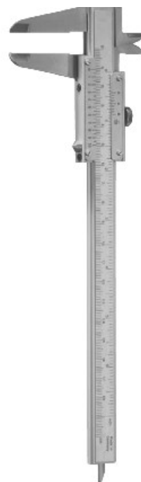
34-831-03 Vernier Caliper Graduated in mm and inches, 150 mm Overall Length 23.5 cm (9 1/4")
